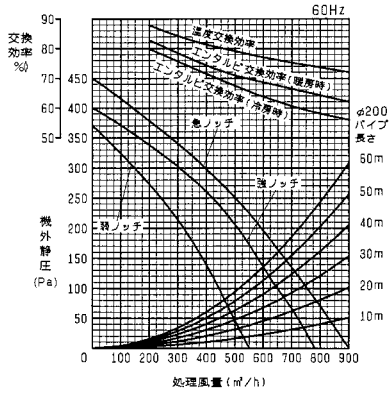
KPI-1001(2)WJ1/KPI-1001(2)SWJ1
