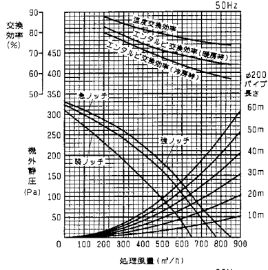
KPI-651(2)WJ1/KPI-651(2)SWJ1
