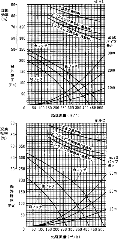
KPI-351(2)WJ1/KPI-351(2)SWJ1
