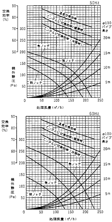
KPI-151(2)WJ1/KPI-151(2)SWJ1
