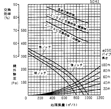
KPI-801(2)WJ1/KPI-801(2)SWJ1
