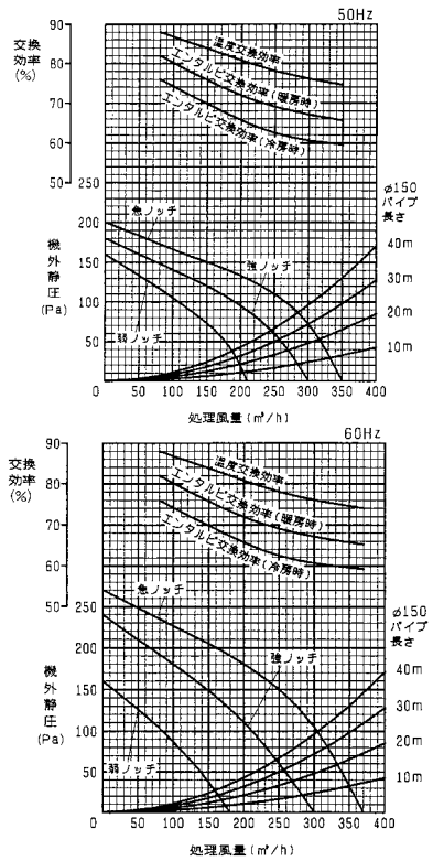
KPI-251(2)WJ1/KPI-251(2)SWJ1
