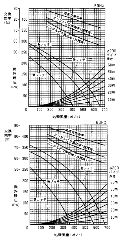
KPI-501(2)WJ1/KPI-501(2)SWJ1
