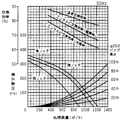
KPI-1001(2)WJ1/KPI-1001(2)SWJ1
