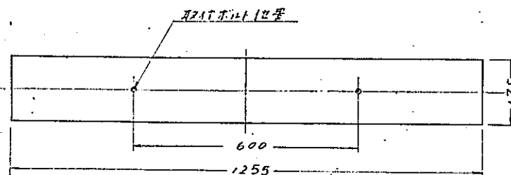
理込穴寸法図( s = \frac{1}{10} )
